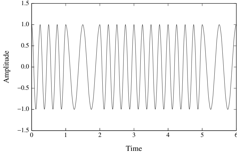
Figure 13: Smooth FSK signal corresponding to the bit sequence (101110).
