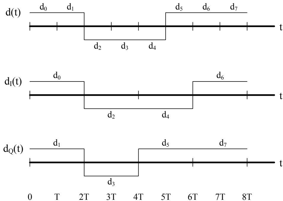
Figure 10: Digital signals used in QPSK modulation.
