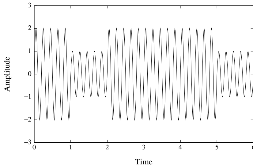
Figure 7: Amplitude modulated signal corresponding to the bit sequence (101110).
